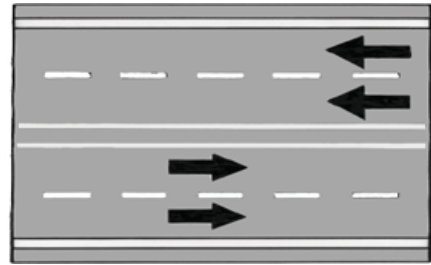
Multi-lane roadway, crossing center or side solid lines permitted to turn or in the event of a breakdown.
